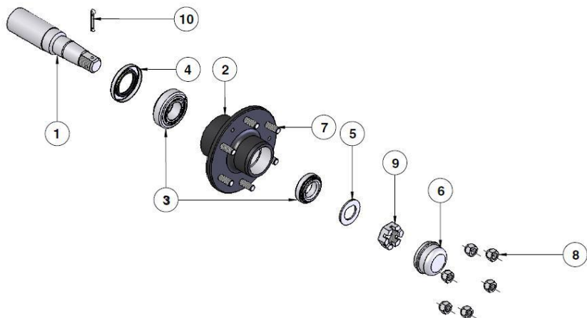
STUB AXLE HP-199B (FAD)
