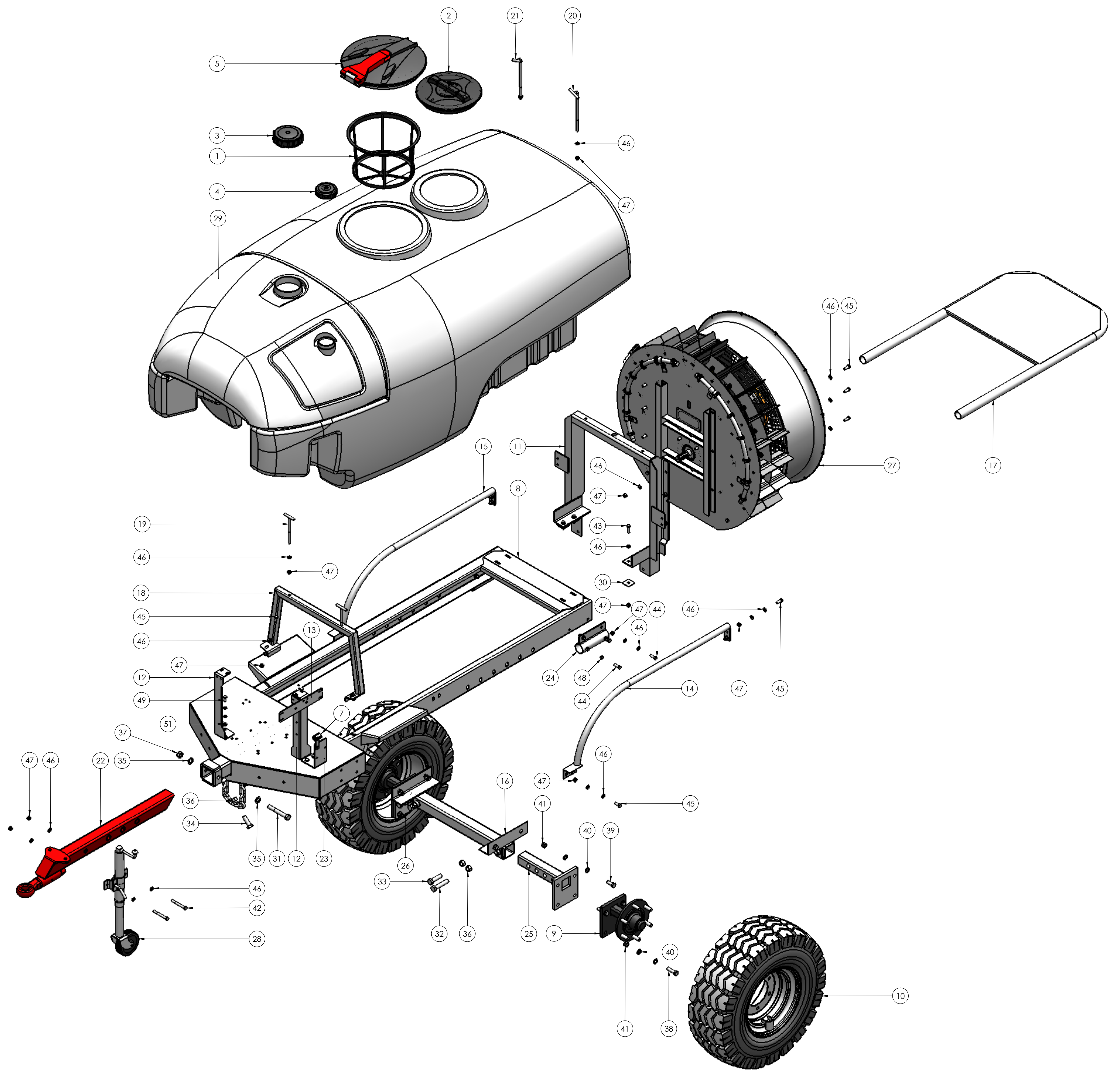
HTP 1500-920SV PARTS ILLUSTRATION THIS DRAWING IS FOR ILLUSTRATION PURPOSE ONLY PLEASE REFER TO THE PARTS LIST.
