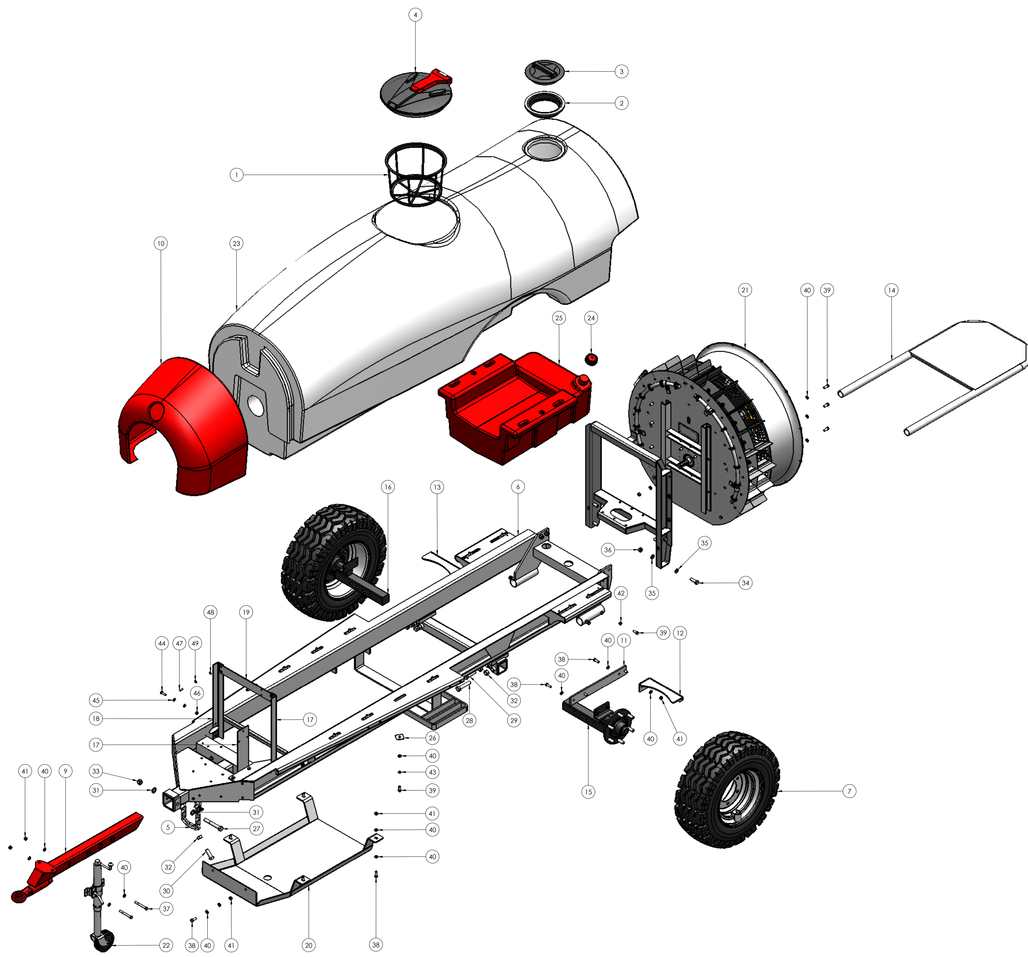
HTPS2000-920SV PARTS ILLUSTRATION THIS DRAWING IS FOR ILLUSTRATION PURPOSE ONLY PLEASE REFER TO THE PARTS LIST.
