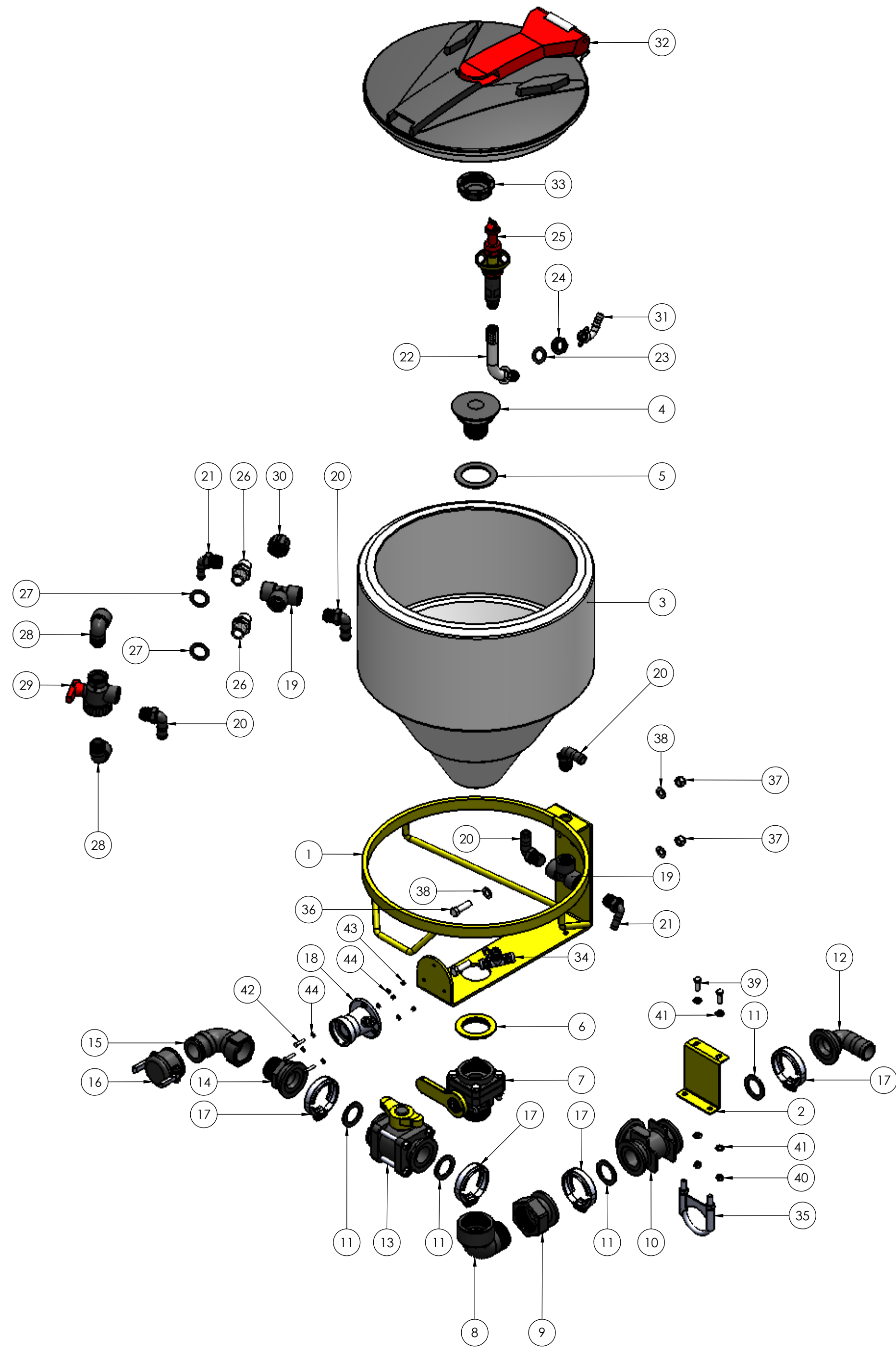
KS-1002 PARTS ILLUSTRATION THIS DRAWING IS FOR ILLUSTRATION PURPOSE ONLY PLEASE REFER TO THE PARTS LIST.
