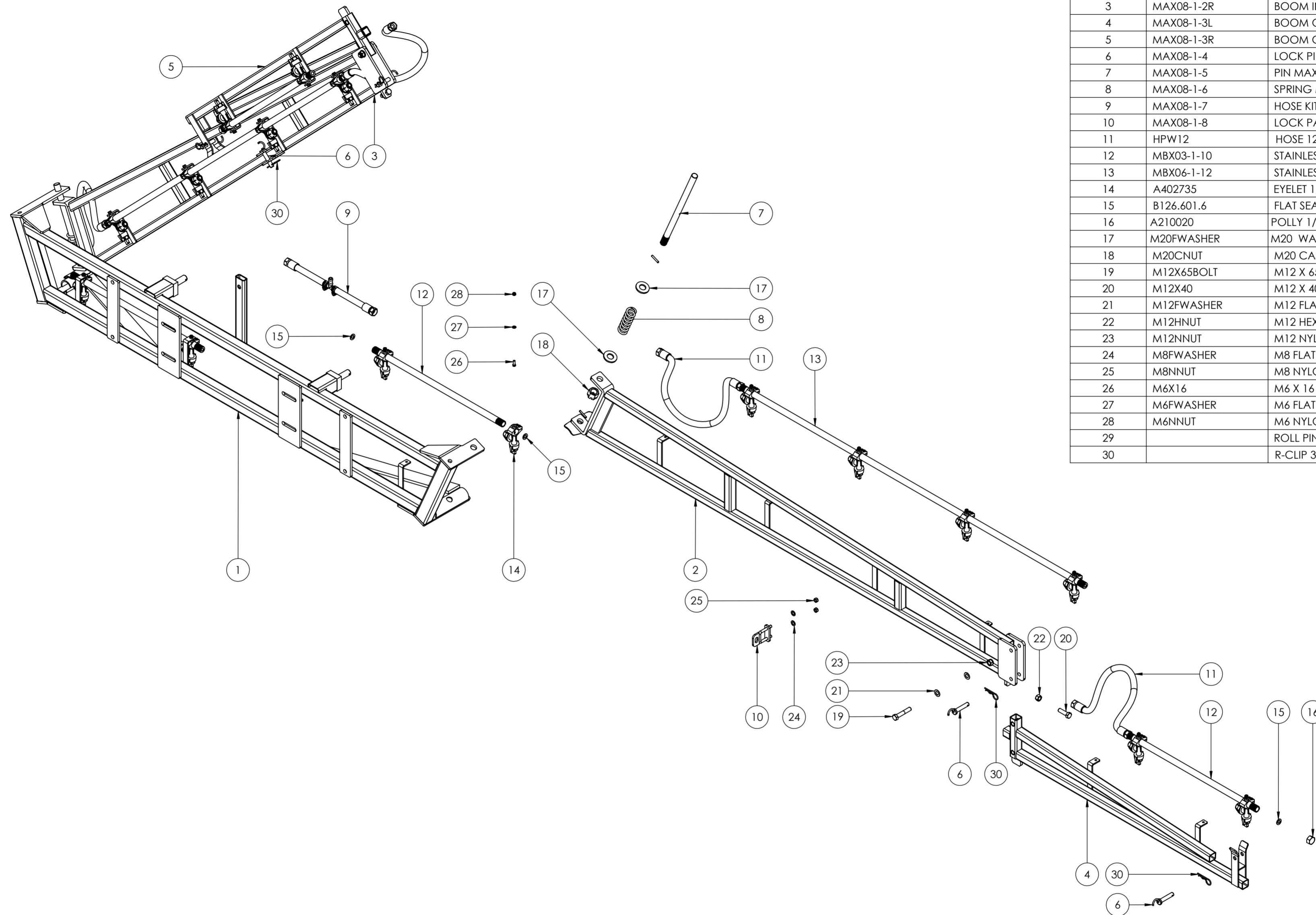
MAX08-1 PARTS ILLUSTRATION THIS DRAWING IS FOR ILLUSTRATION PURPOSE ONLY PLEASE REFER TO THE PARTS LIST.
