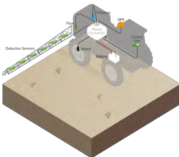
Figure 3-1 Electrical system overview
