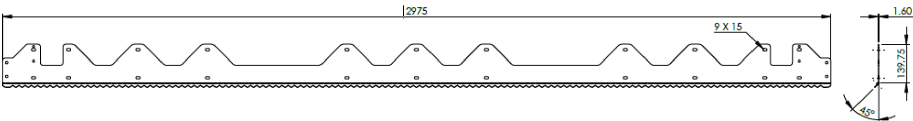
1 NOZZLE PROTECTION 2975 MATERIAL : 1.6 M.S. PLATE
