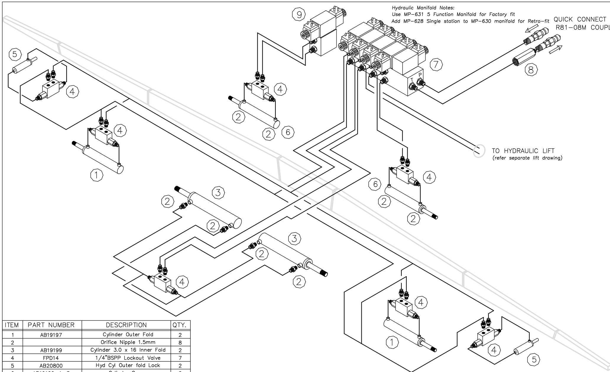
33/36m BOOM WINGLIFT & OUTER WING FOLD OPTION
