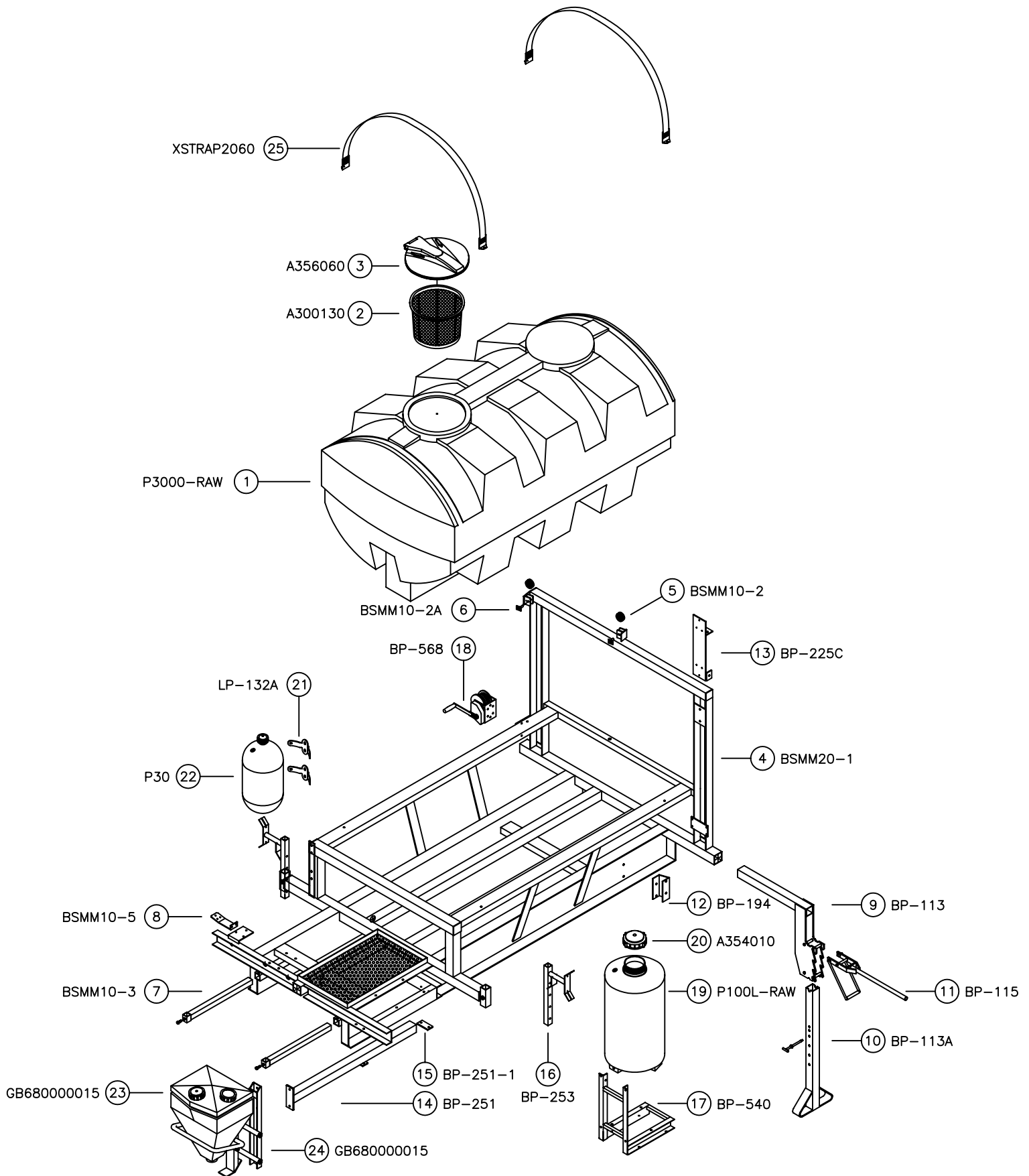
2000LT BRUMBY CHASSIS ASSEMBLY
