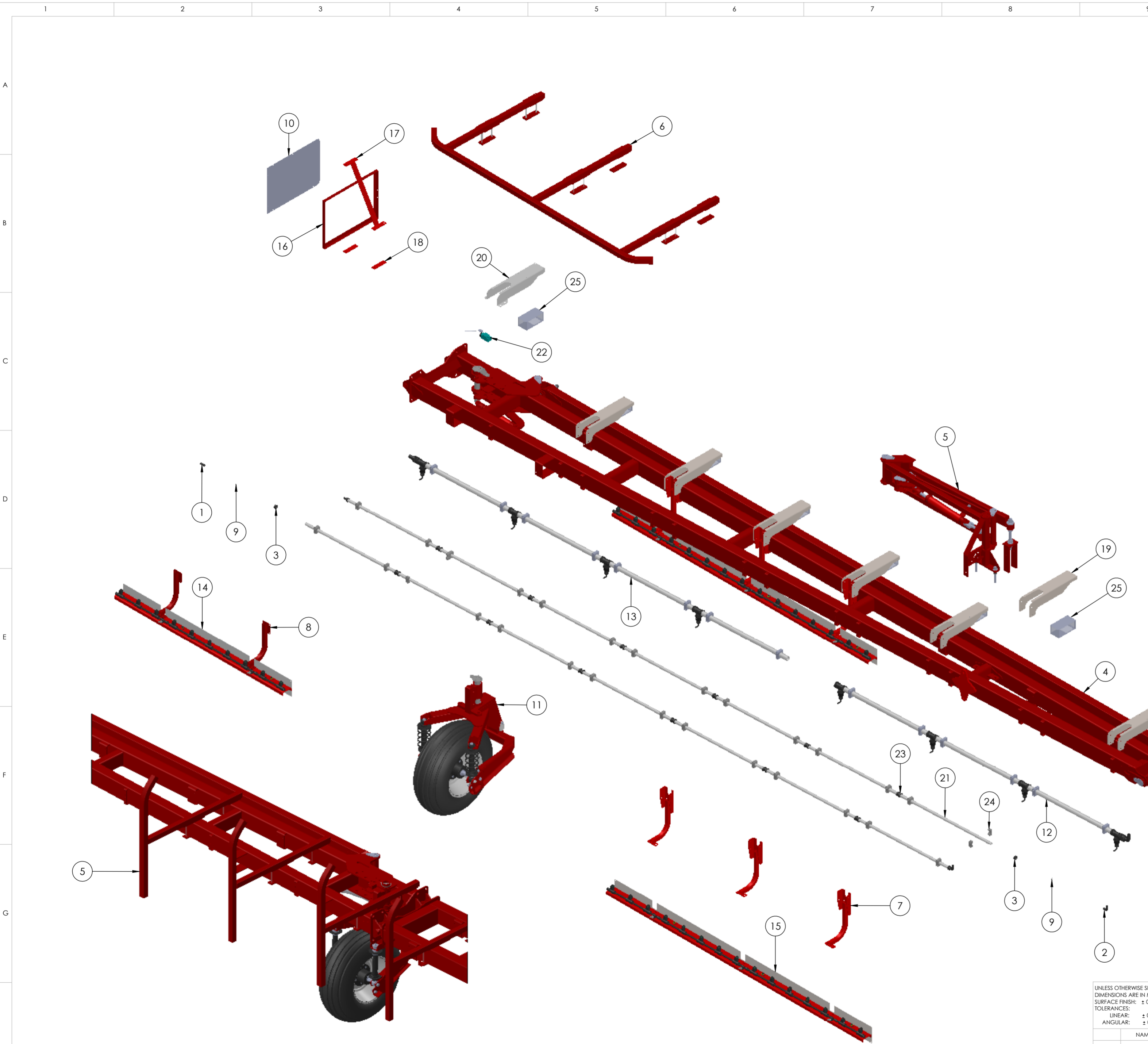
MOUNTING OF AB243000-700A ON OPPOSITE ARM
