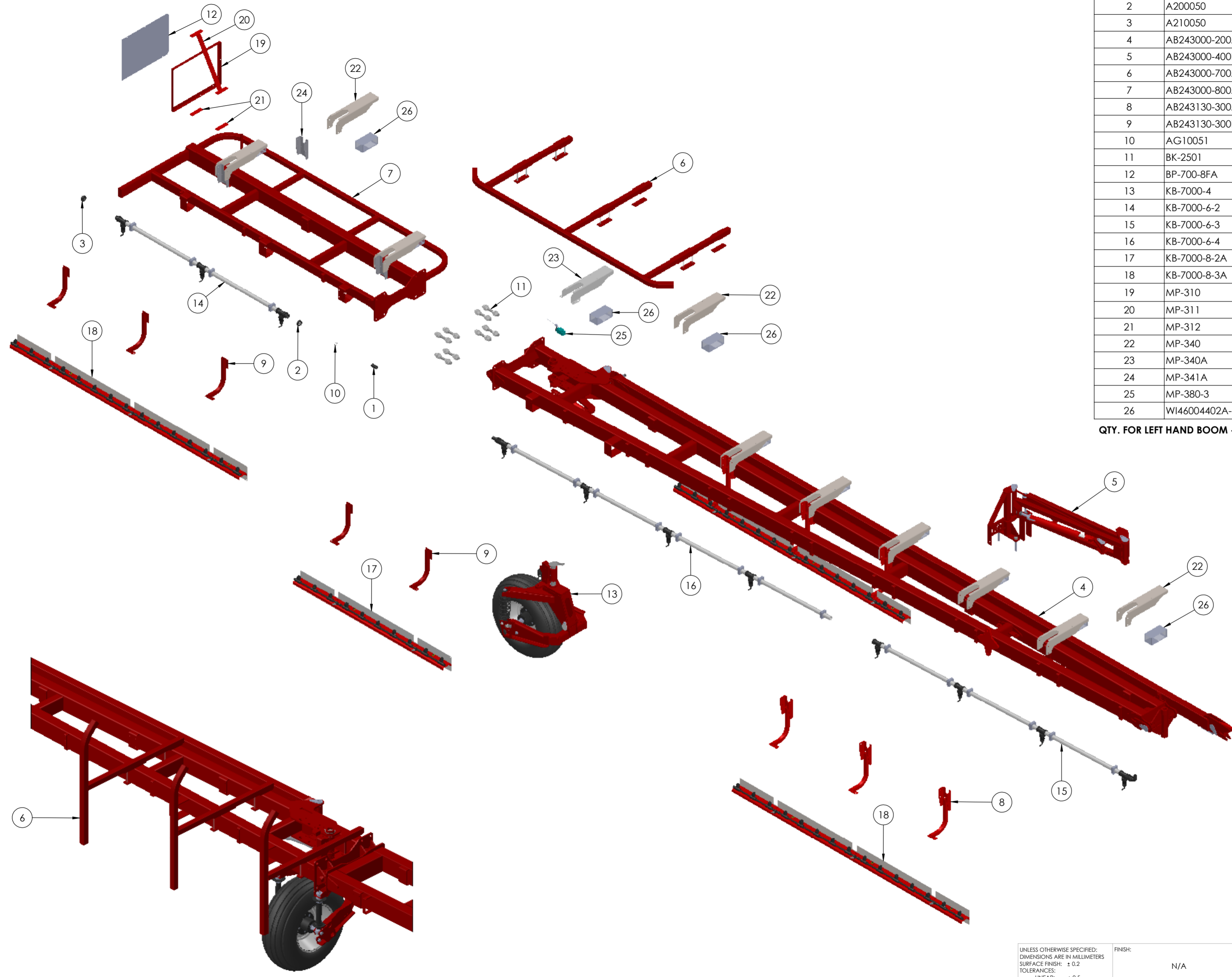
MOUNTING OF AB243000-700A ON OPPOSITE ARM
