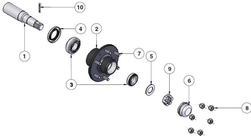
STUB AXLE HP-199F
