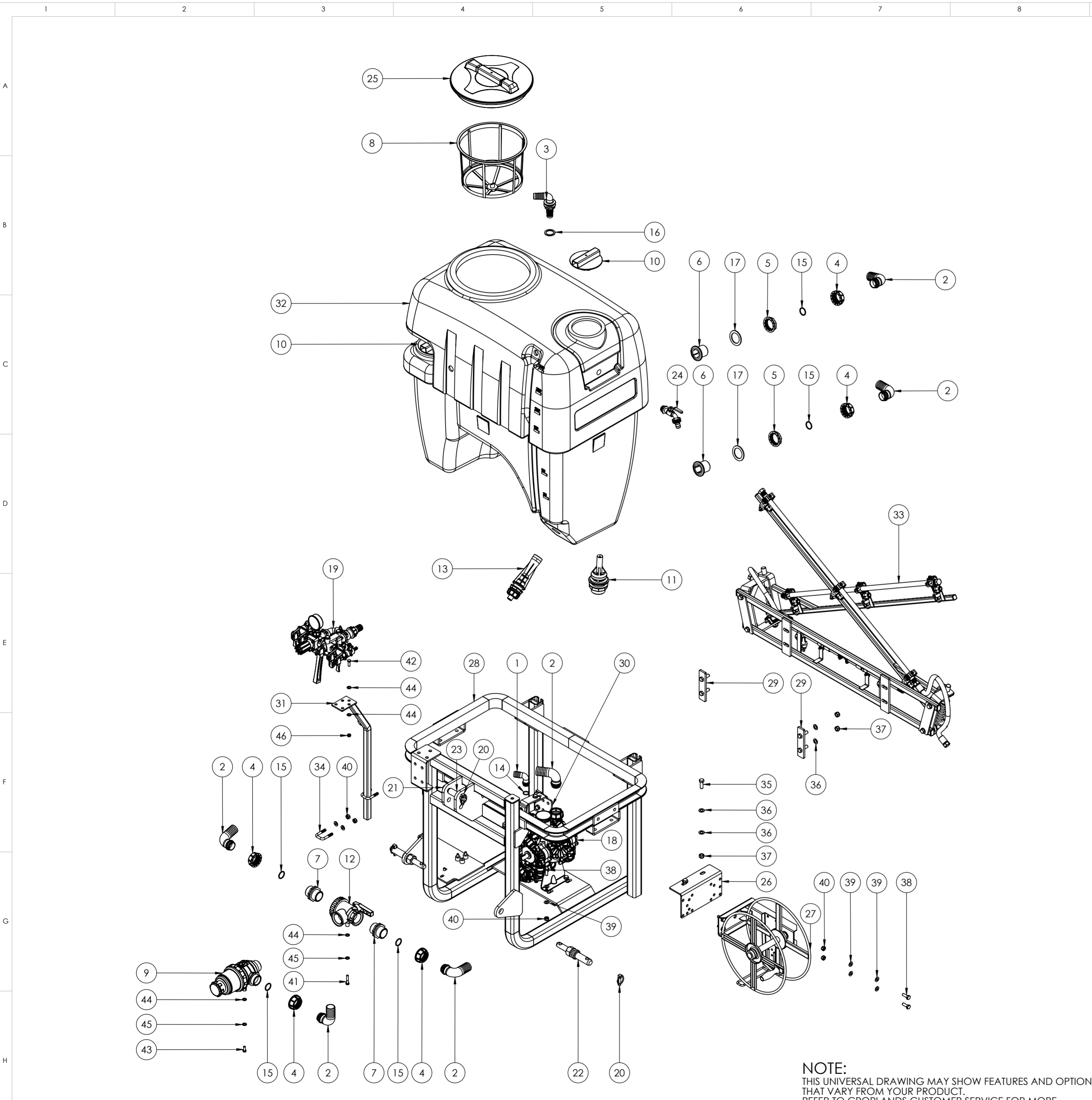
LA300/MBX04 PARTS ILLUSTRATION THIS DRAWING IS FOR ILLUSTRATION PURPOSE ONLY PLEASE REFER TO THE PARTS LIST.
