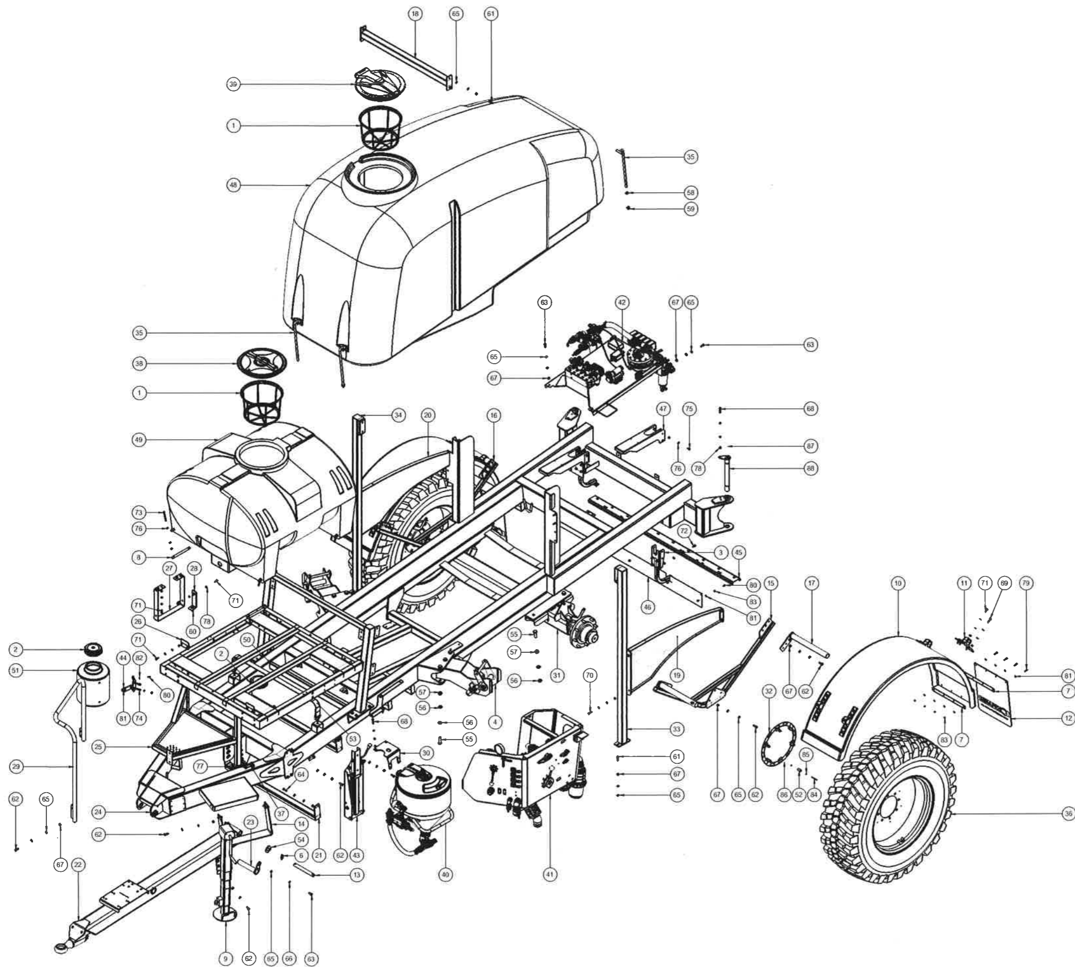
WEEDIT 6000 PARTS ILLUSTRATION THIS DRAWING IS FOR ILLUSTRATION PURPOSE ONLY PLEASE REFER TO THE PARTS LIST.
